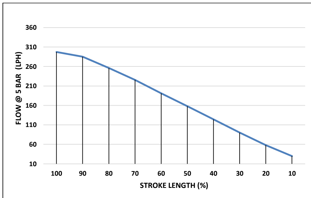
EDOSE MAX 300 LPH STROKE LENGTH Vs FLOW
