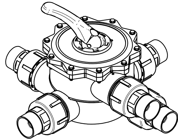
50nb SIDE MOUNT FILTER MULTIPOINT VALVE GENERAL ASSEMBLY
